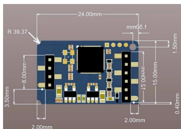
Fig. 2: Schematic diagram for radar module frame
