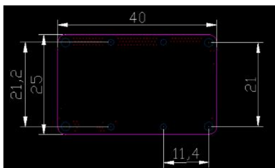
Fig. 2: Schematic diagram for radar module frame
