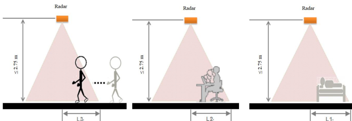
Fig. 8 Top mounting
