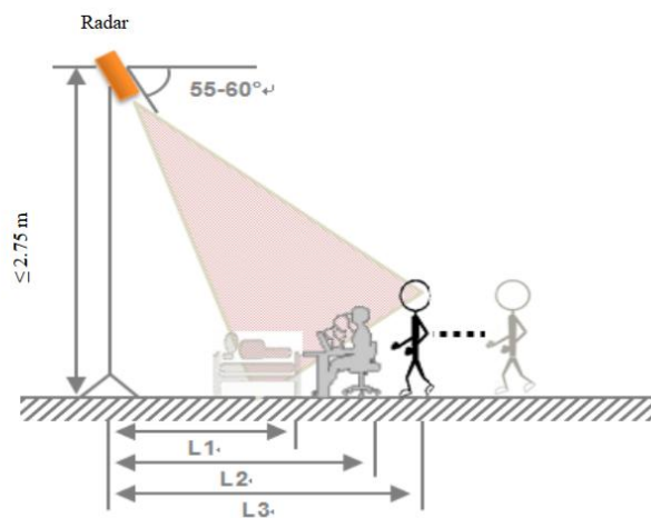
Fig. 7 Look-down mounting
