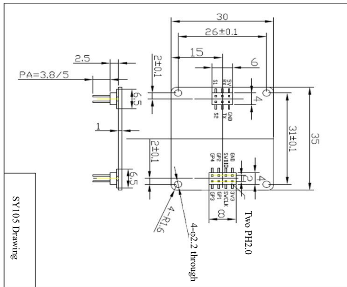
Fig. 2: Schematic diagram for radar module frame
