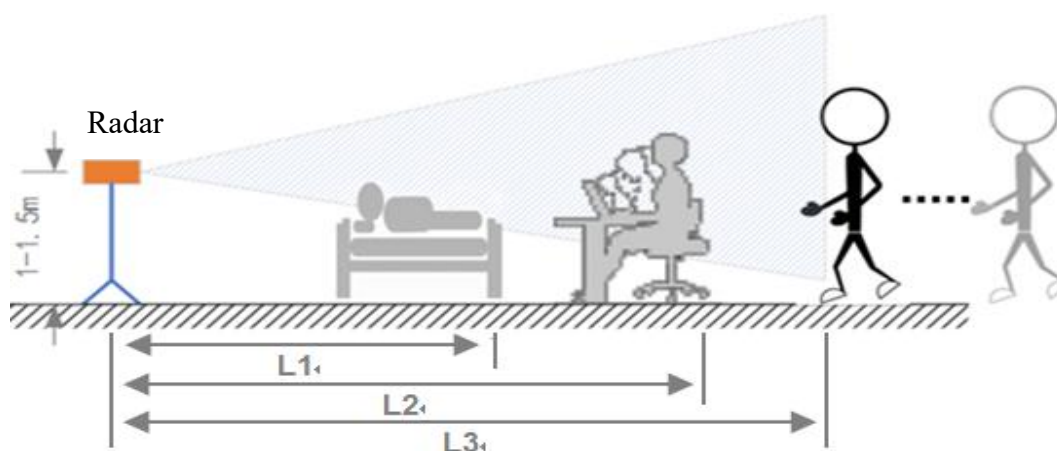
Fig. 7 Diagram of Side Mounting
