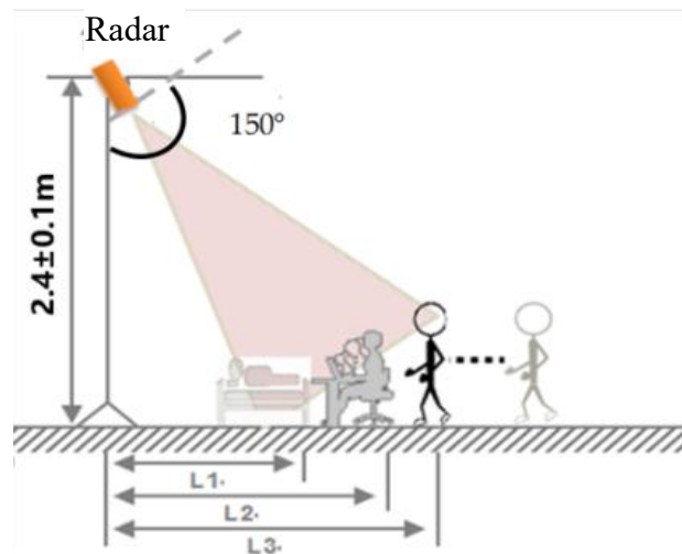
Fig. 7 Diagram of inclined mounting
