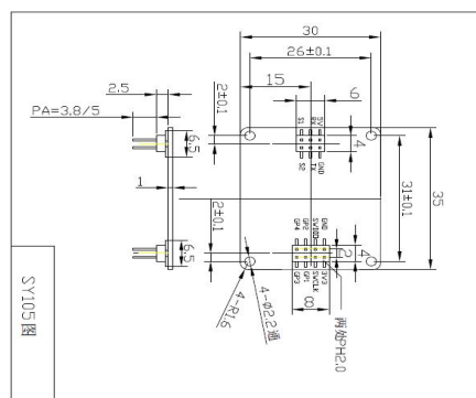
Fig. 2 Schematic diagram for radar module frame
