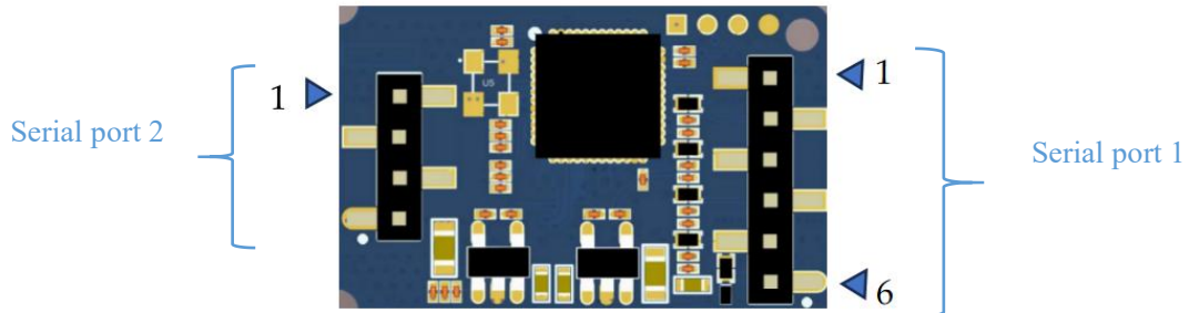
Fig. 3 Radar Pins Explanation
