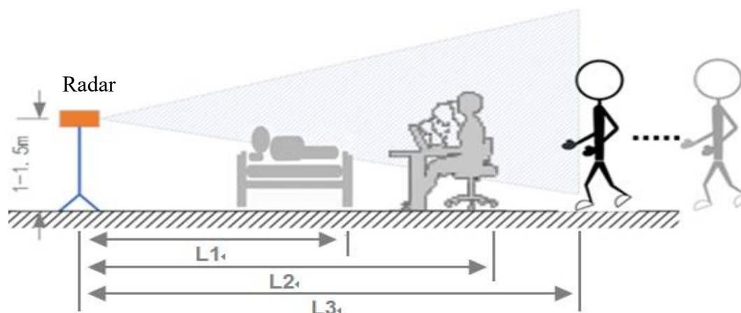
Fig. 7 Diagram of Side Mounting
